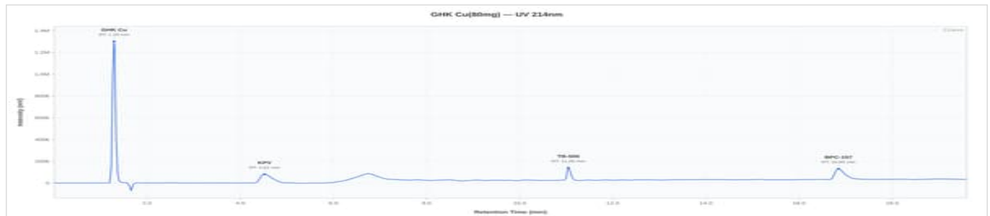
KLOWS-8 80mg - K8026060201: UV Chromatogram
