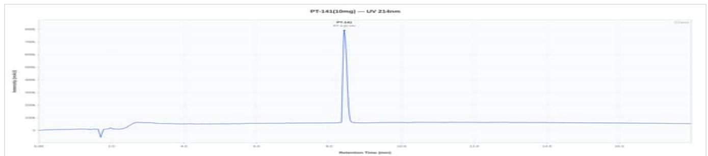
PT-141 10mg - P41260623: UV Chromatogram
