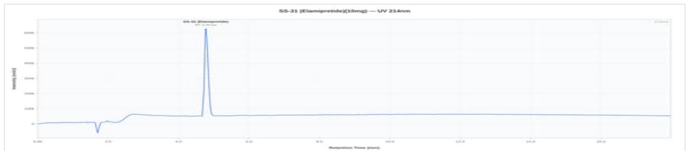
SS-31 10mg - 2S10260614: UV Chromatogram
